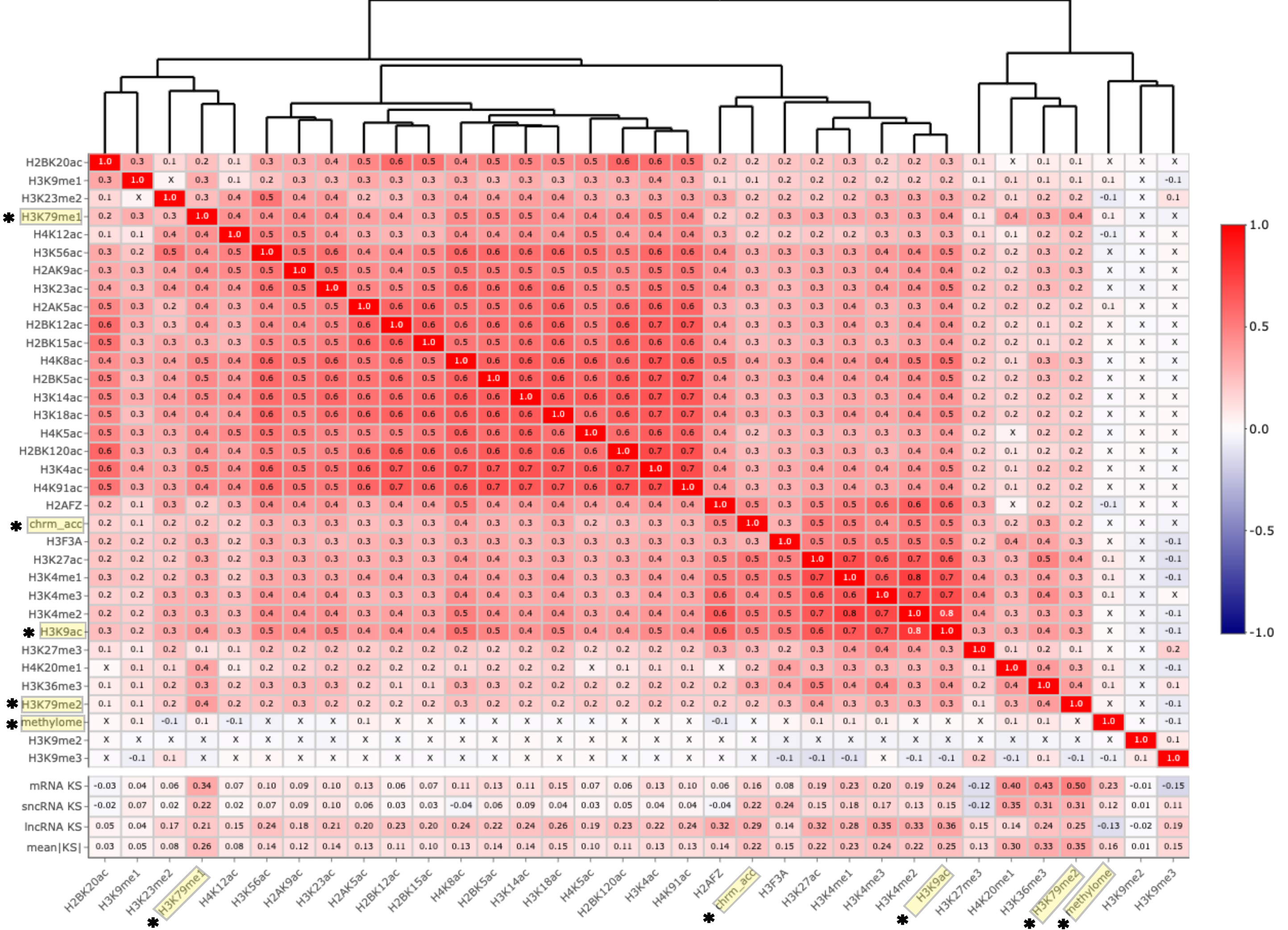
Supplementary Figure S8. Correlation matrix of epigenetic features. Spearman correlation of histone and DNA modifications for mRNA, sncRNA and lncRNA sequences. Positively correlated features are displayed in red and negatively correlated features in blue. Spearman's Rho was used to determine the significance of each correlation, which were corrected for multiple testing using a Benjamini-Hochberg (BH) correction. Non-significant correlations with a p-value > 0.05 have been marked with a cross. At the bottom of the plot, KS statistics are included for each gene type as well as a mean |KS| for overall comparison
